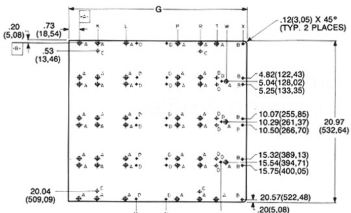
12U Side Plate
