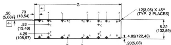
3U Side Plate
