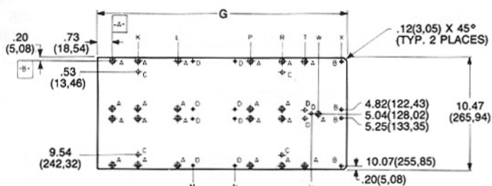
6U Side Plate
